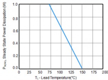
Figure 5 - Steady State Power Derating Curve
